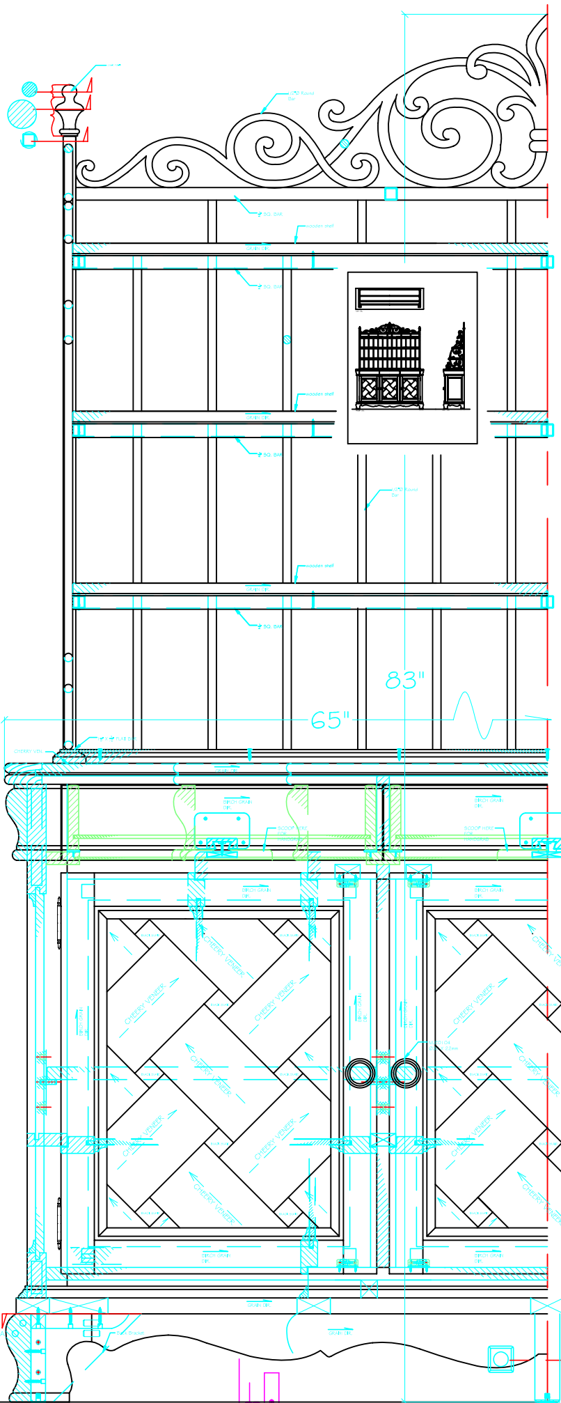
FRONT VIEW
